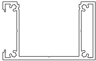
KESC8050 U Channel - Box (50 x 80mm) - Fits 50mm Geos
